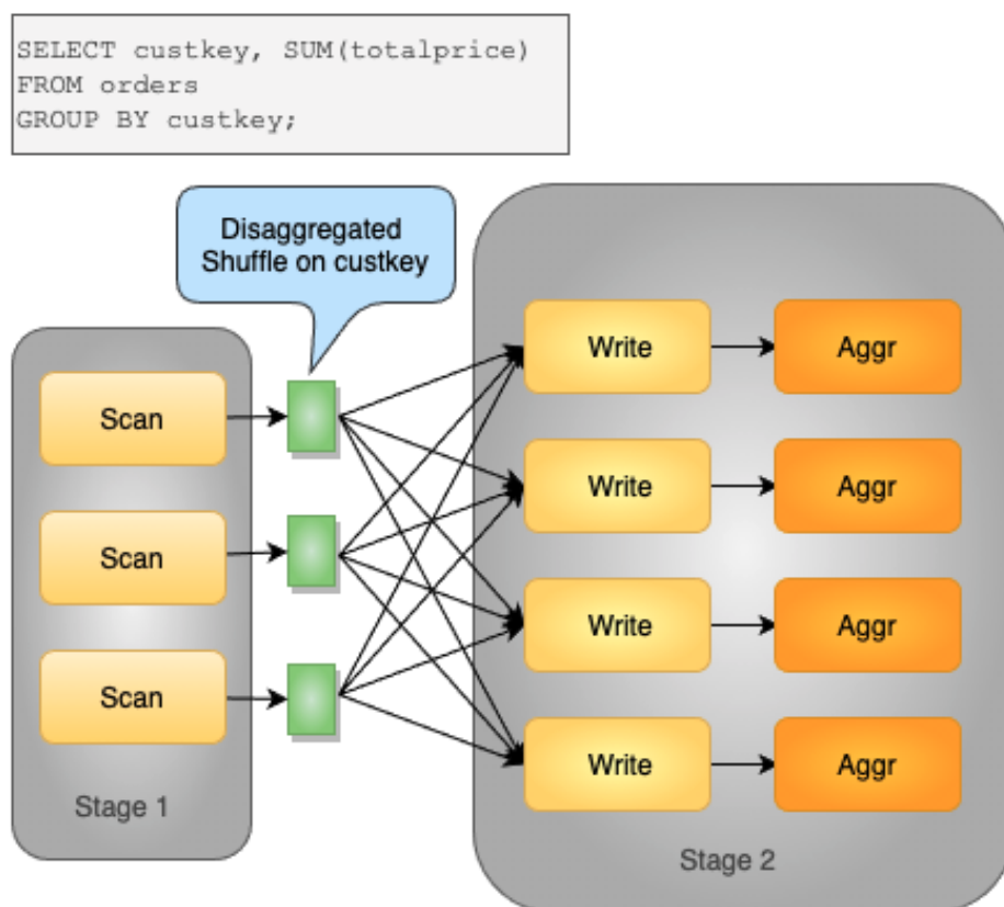
Presto Evaluation Library on Spark Runtime
